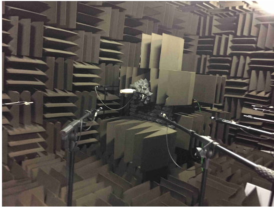
(a) The isolated jet noise experiment setup: microphones are located at 50D to the jet nozzle centre, with observer angle ranging from 30° to 120° to the jet centreline.
